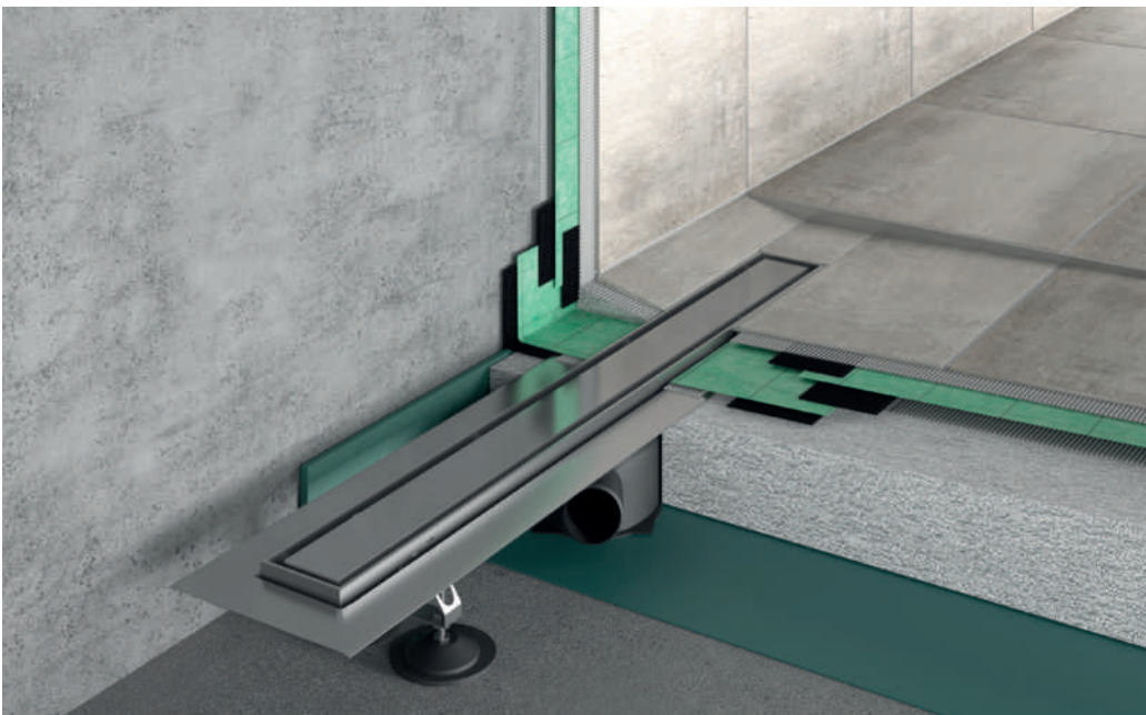
Primary and secondary drainage with PROCHANNELS-line (see p. 14-17)
