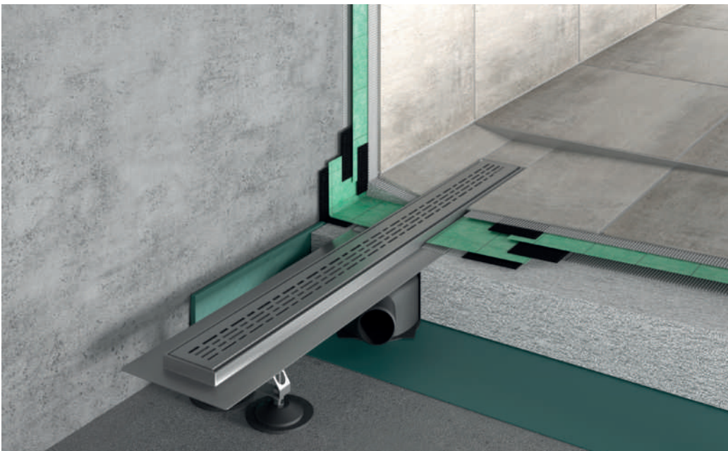
Proven primary drainage with PROCHANNELp-line (see p. 18-19)
